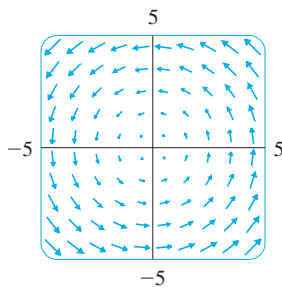
FIGURE 6 \mathbf{F}(x, y) = \langle -y, x \rangle
